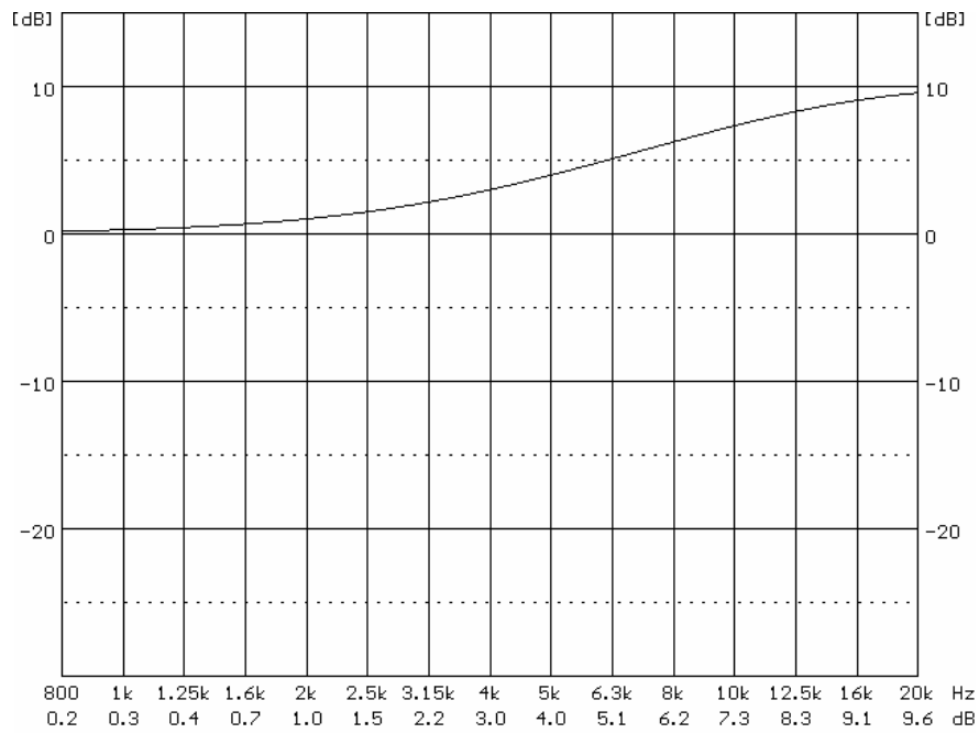
Frequency characteristics of ENVIRONMENTAL filter
