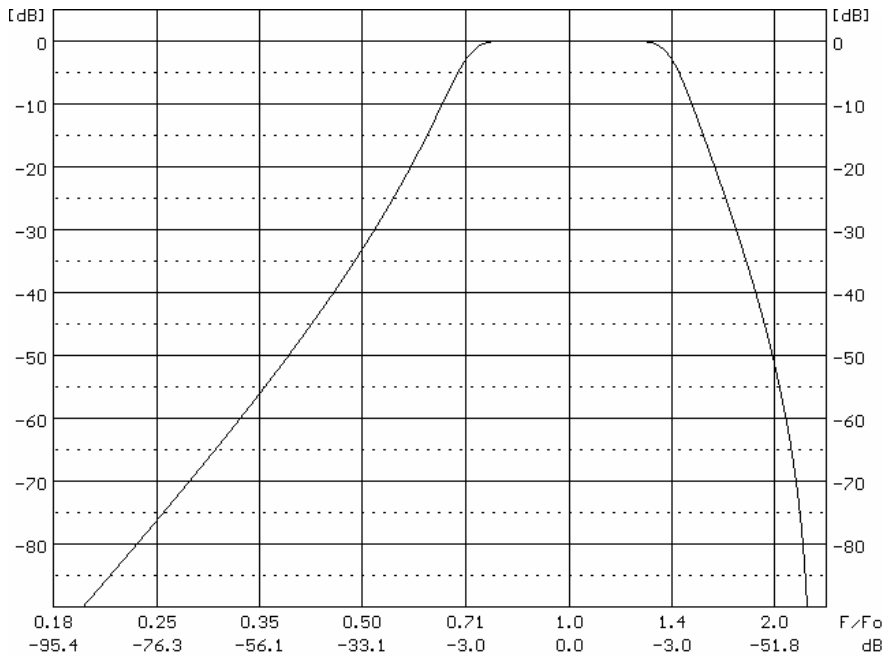
Characteristics of the exemplary digital 1/1 OCTAVE filter implemented in the instrument
