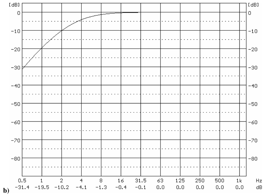
Full (a) and low band (b) frequency characteristics of Z filter implemented in the instrument
