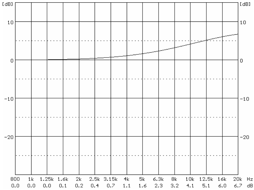
Frequency characteristics of AIRPORT filter
